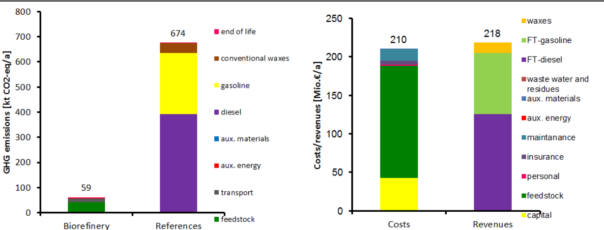
Figure 69: Estimated greenhouse gas emissions of biorefinery and reference products
