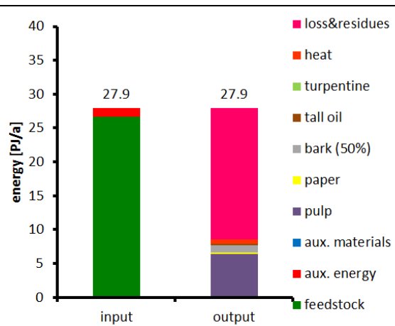
Figure 13: Energy balance of biorefinery plant
