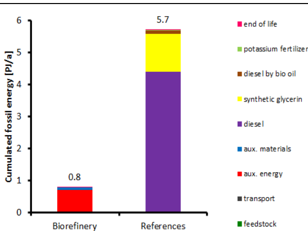
Figure 57: Estimated cumulated fossil energy demand of biorefinery and reference products
