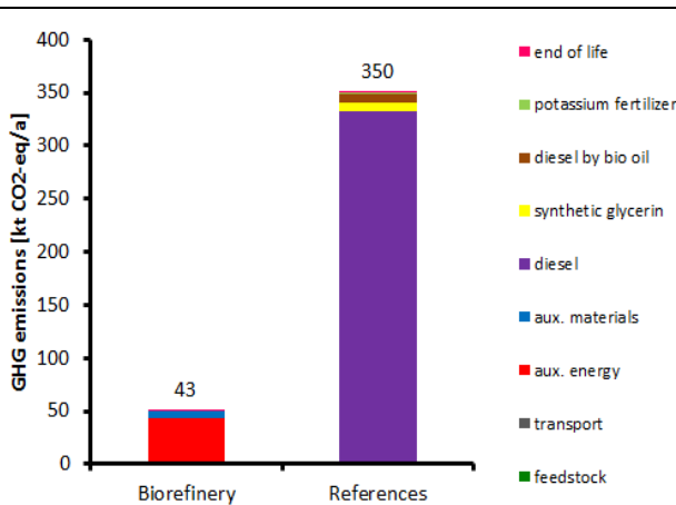
Figure 59: Estimated greenhouse gas emissions of biorefinery and reference products
