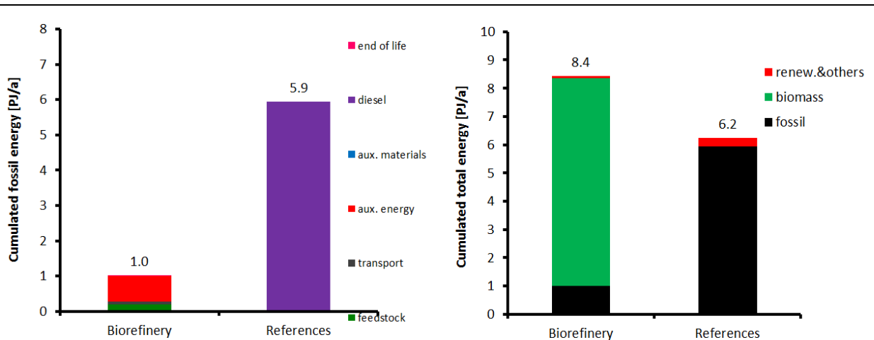
Figure 77: Estimated cumulated fossil energy demand of biorefinery and reference products
