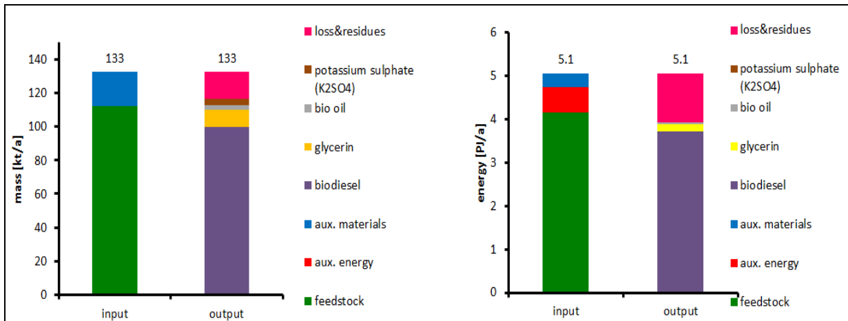
Figure 52: Mass balance of biorefinery plant
