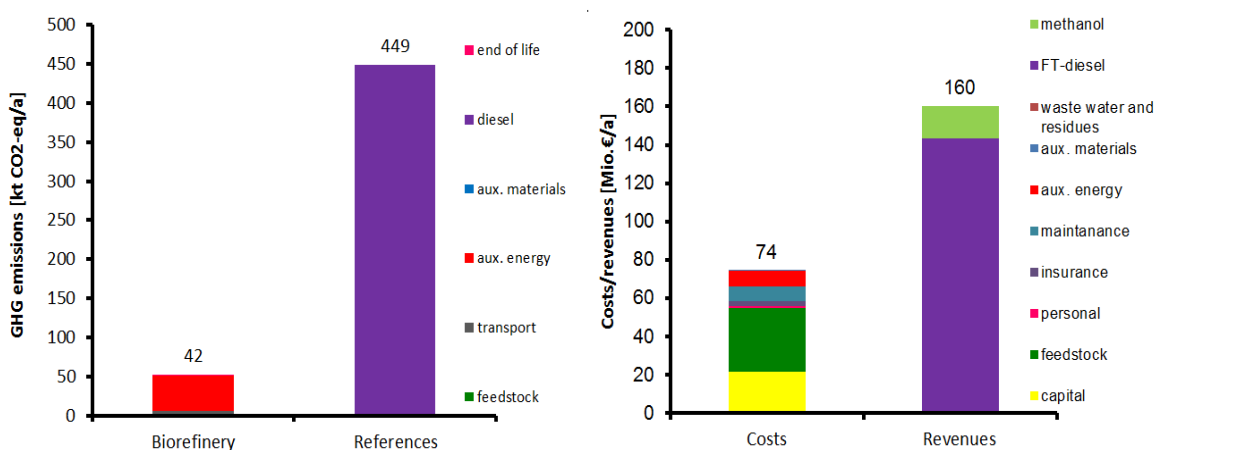
Figure 79: Estimated greenhouse gas emissions of biorefinery and reference products
